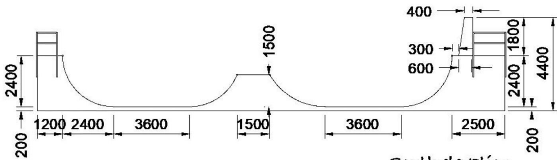
South elevation
